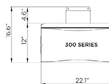
FRONT PROFILE (WITHOUT HEAT DEFLECTOR)
