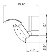
SIDE PROFILE (WITH HEAT DEFLECTOR)
