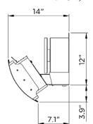
SIDE PROFILE (WITHOUT HEAT DEFLECTOR)
